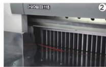
垫刀条顶出装盒 Ejecting device of knife holder
